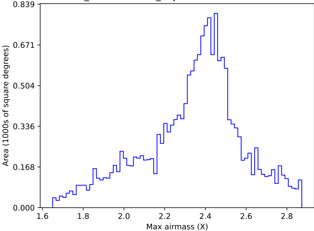
weather_cloudso36v3.4_10yrs WFD r band: Max airmass
