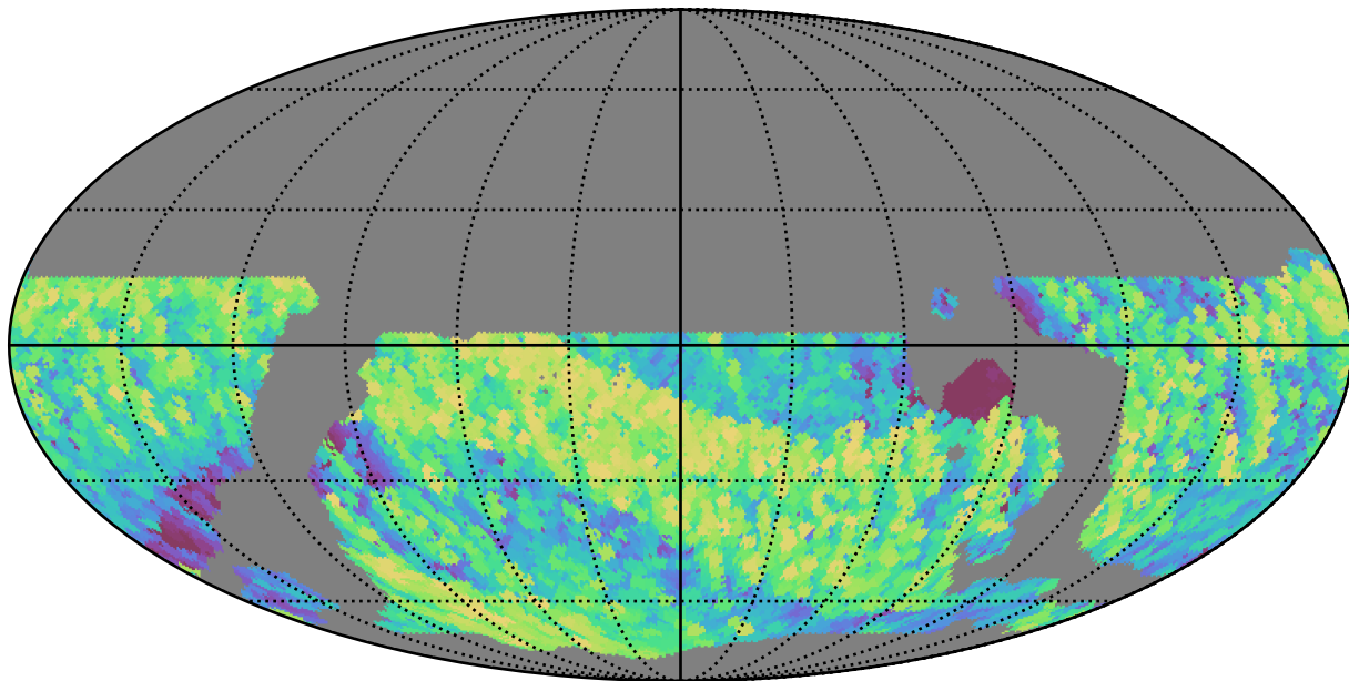
weather_cloudso36v3.4_10yrs WFD i band: Max airmass
