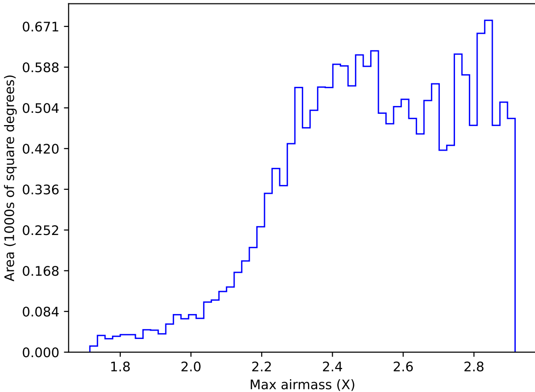
weather_cloudso36v3.4_10yrs WFD i band: Max airmass
