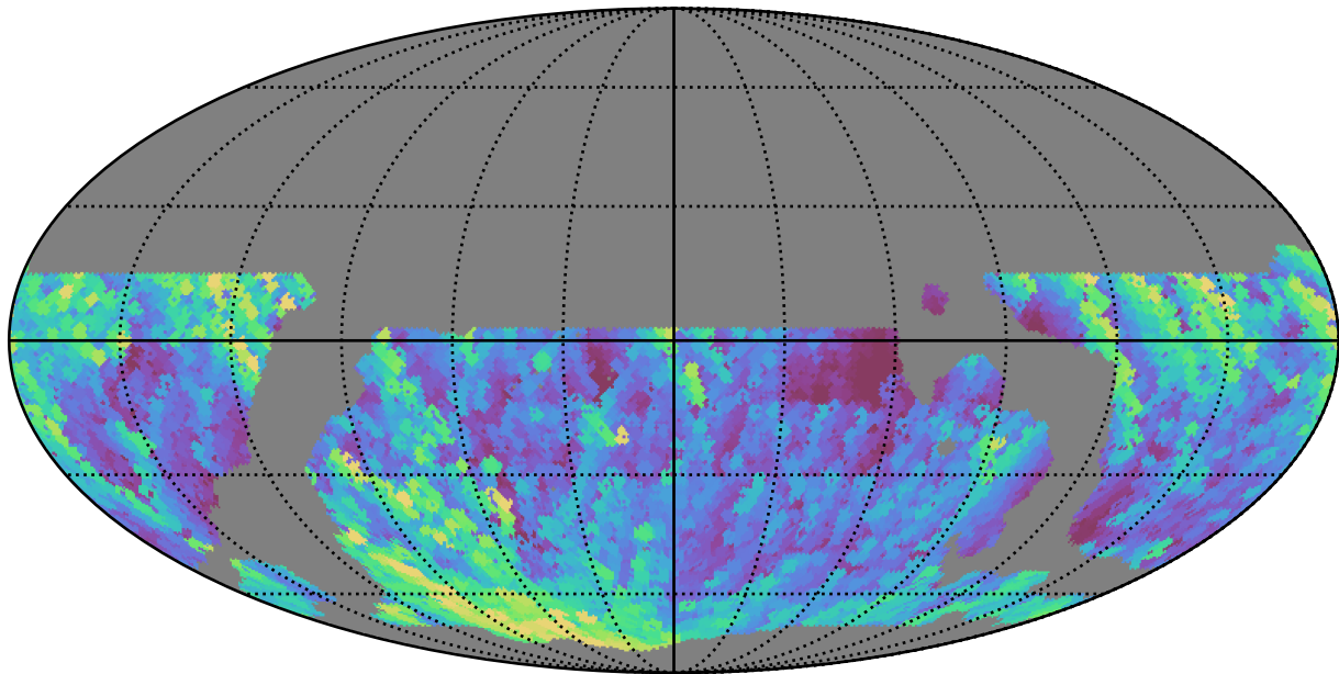
weather_cloudso36v3.4_10yrs WFD g band: Max airmass
