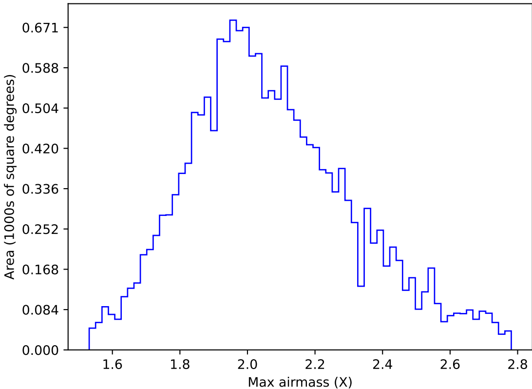
weather_cloudso36v3.4_10yrs WFD g band: Max airmass
