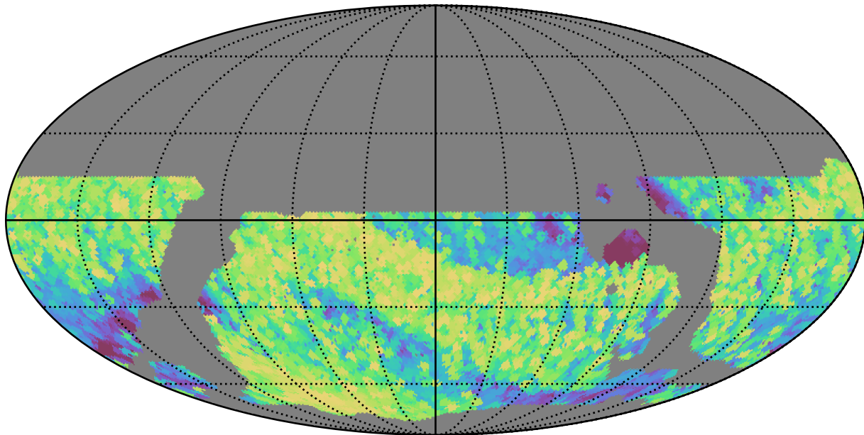
weather_cloudso36v3.4_10yrs WFD all bands: Max airmass
