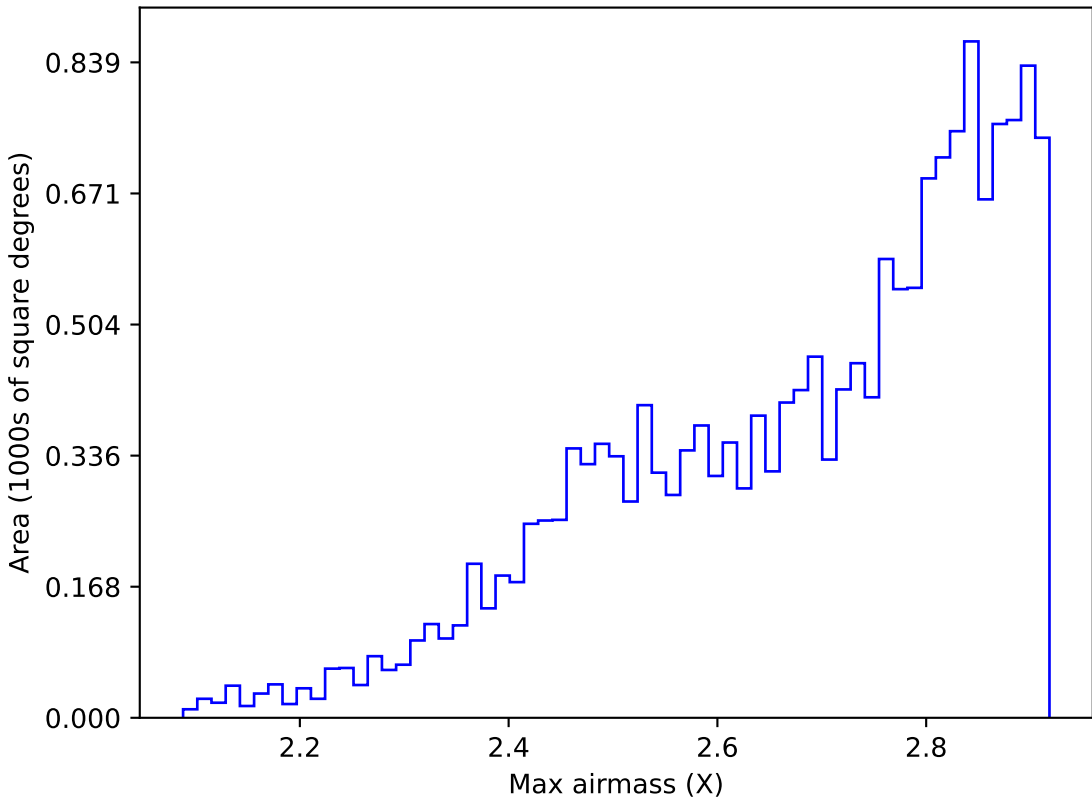
weather_cloudso36v3.4_10yrs WFD all bands: Max airmass
