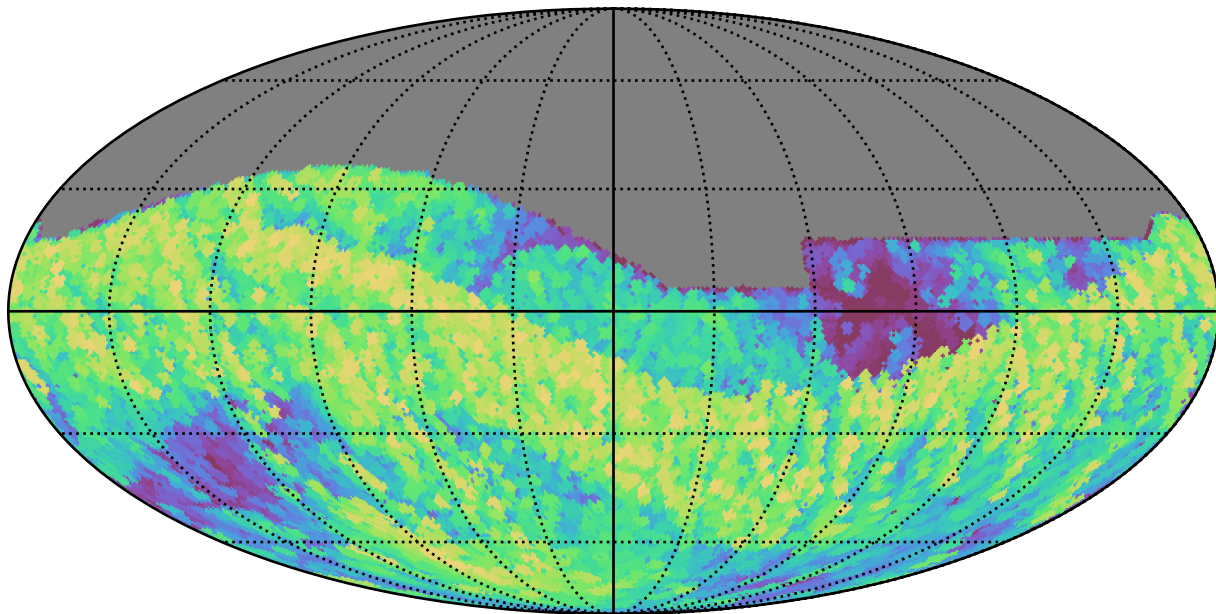
weather_cloudso36v3.4_10yrs All sky z band: Max airmass
