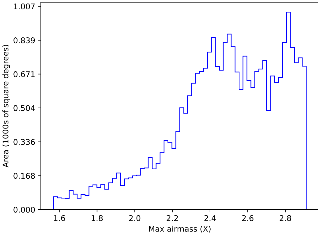
weather_cloudso36v3.4_10yrs All sky z band: Max airmass
