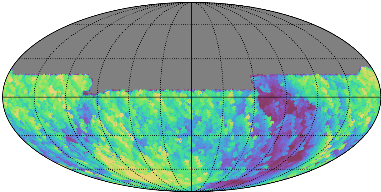
weather_cloudso36v3.4_10yrs All sky y band: Max airmass
