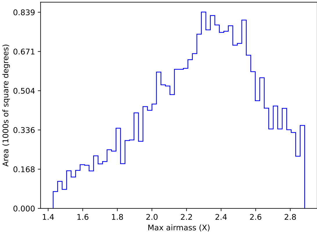
weather_cloudso36v3.4_10yrs All sky y band: Max airmass
