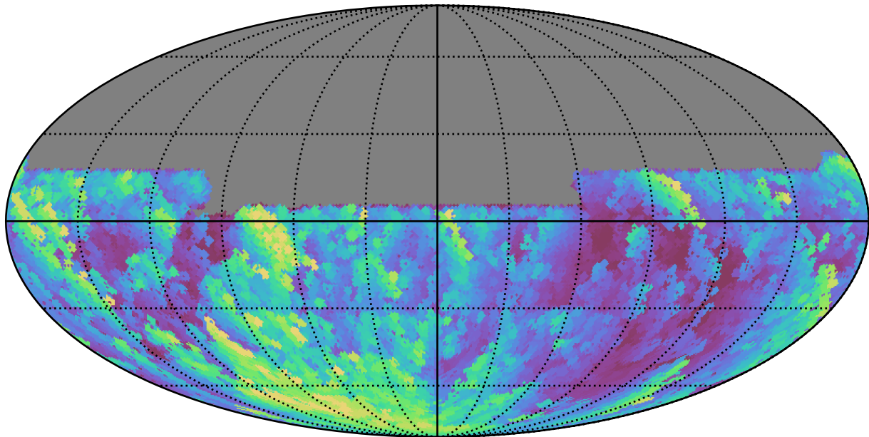
weather_cloudso36v3.4_10yrs All sky u band: Max airmass
