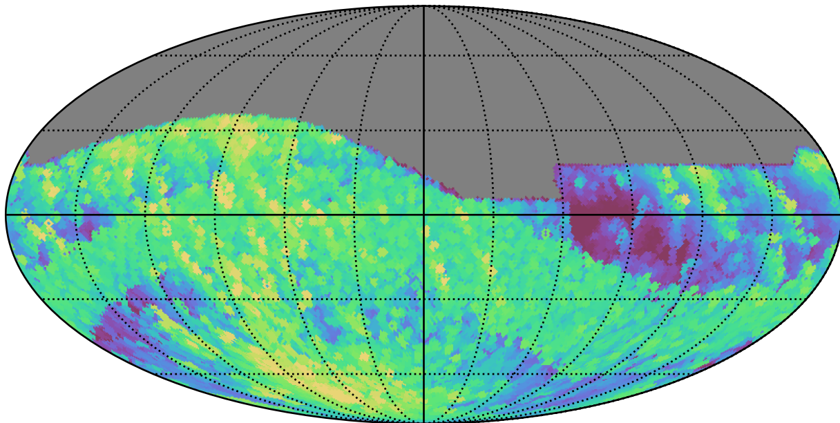
weather_cloudso36v3.4_10yrs All sky r band: Max airmass
