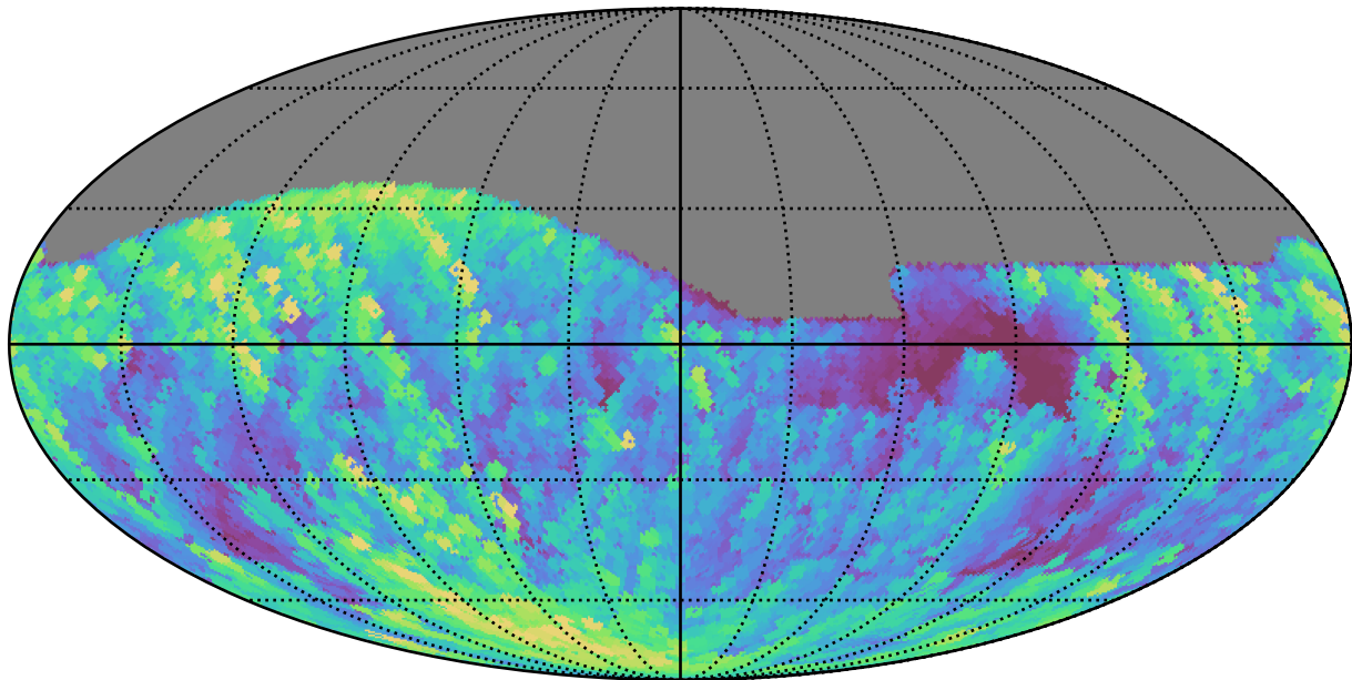
weather_cloudso36v3.4_10yrs All sky g band: Max airmass
