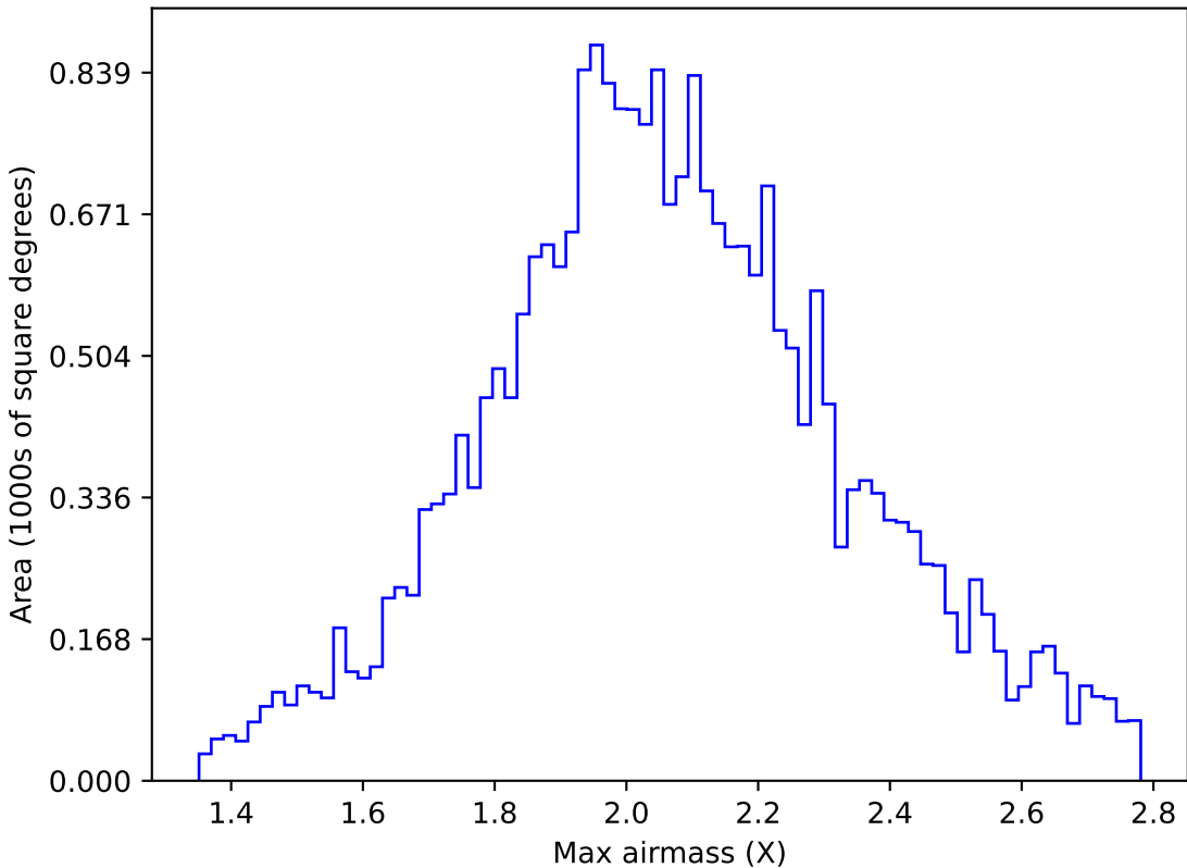
weather_cloudso36v3.4_10yrs All sky g band: Max airmass
