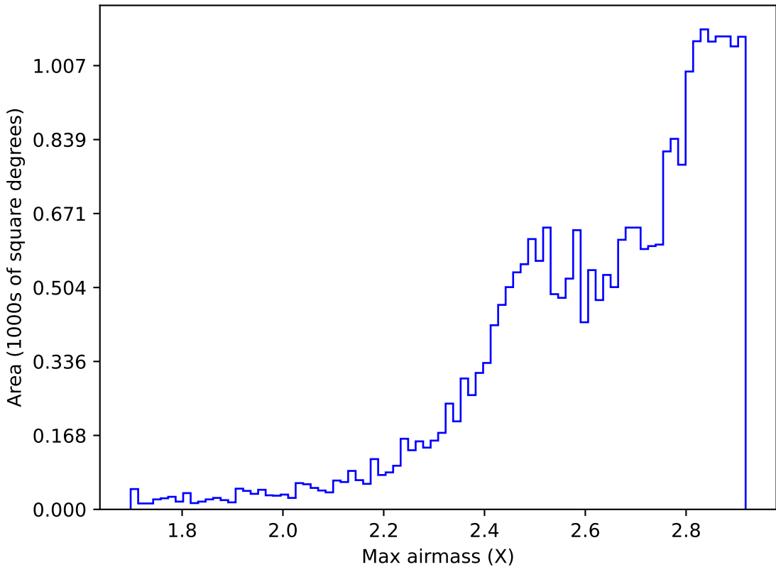
weather_cloudso36v3.4_10yrs All sky all bands: Max airmass
