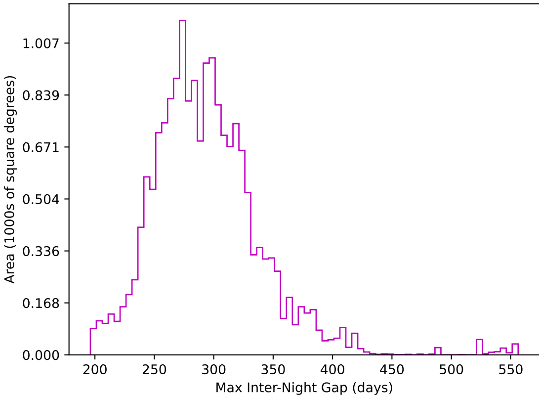
weather_cloudso36v3.4_10yrs WFD z band: Max Inter-Night Gap
