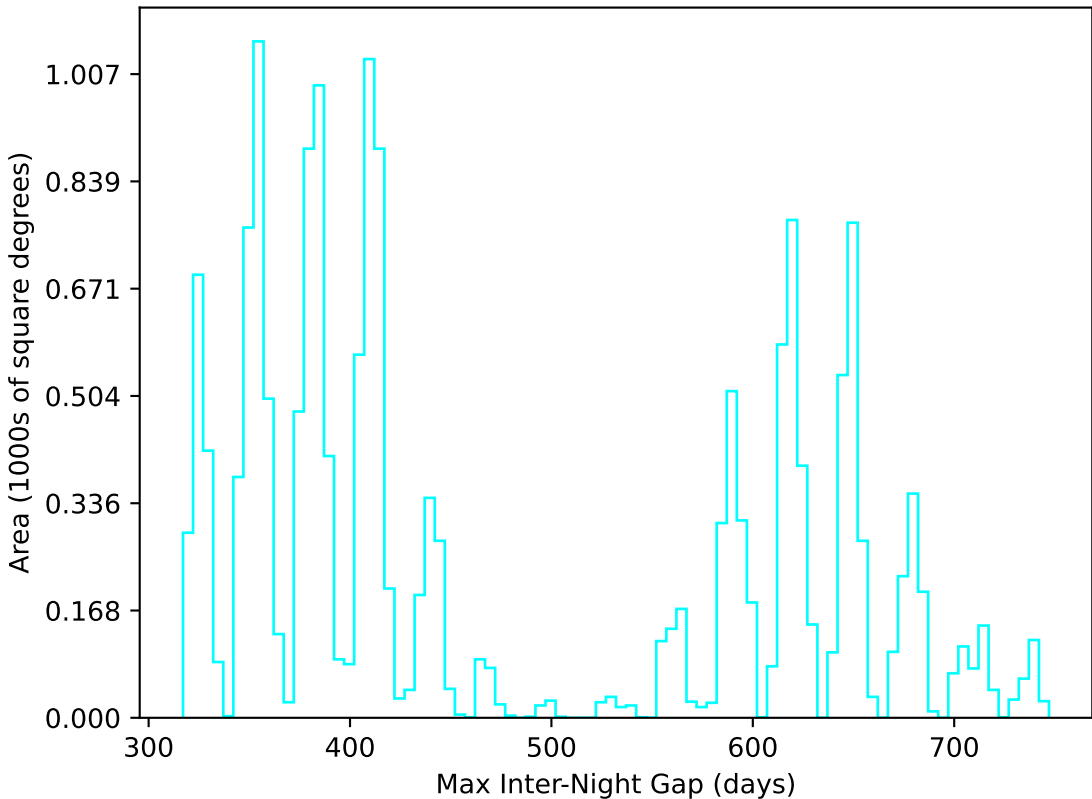
weather_cloudso36v3.4_10yrs WFD u band: Max Inter-Night Gap
