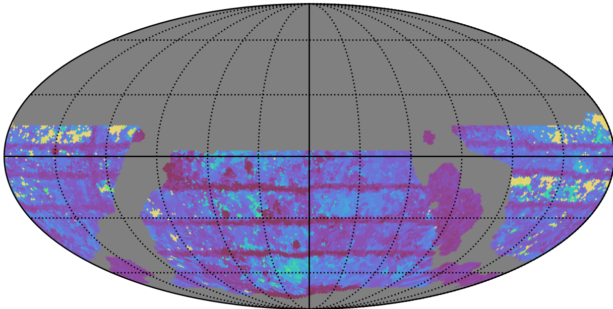
weather_cloudso36v3.4_10yrs WFD i band: Max Inter-Night Gap
