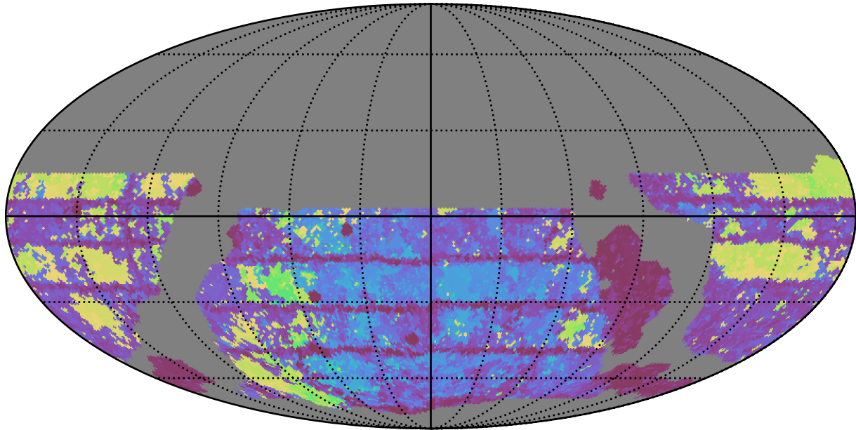
weather_cloudso36v3.4_10yrs WFD g band: Max Inter-Night Gap
