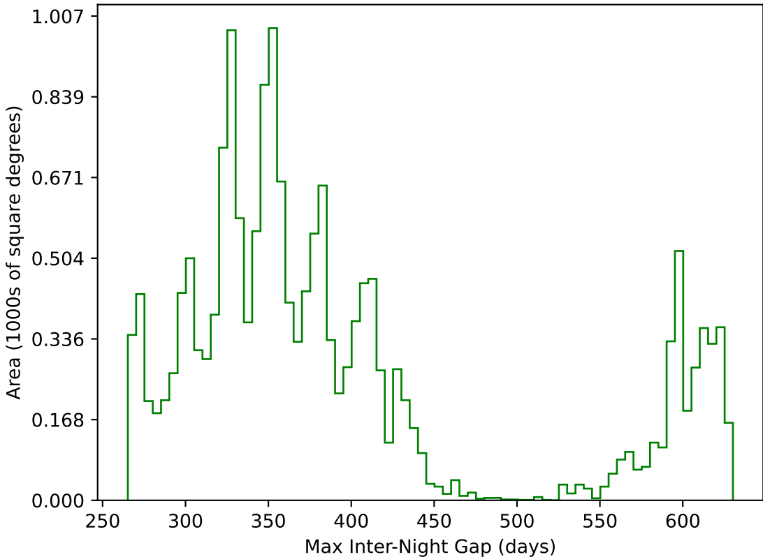
weather_cloudso36v3.4_10yrs WFD g band: Max Inter-Night Gap
