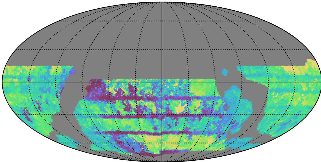
weather_cloudso36v3.4_10yrs WFD all bands: Max Inter-Night Gap
