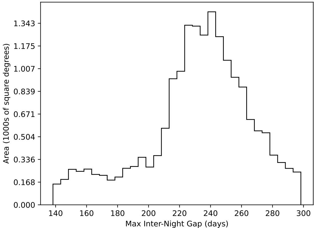
weather_cloudso36v3.4_10yrs WFD all bands: Max Inter-Night Gap
