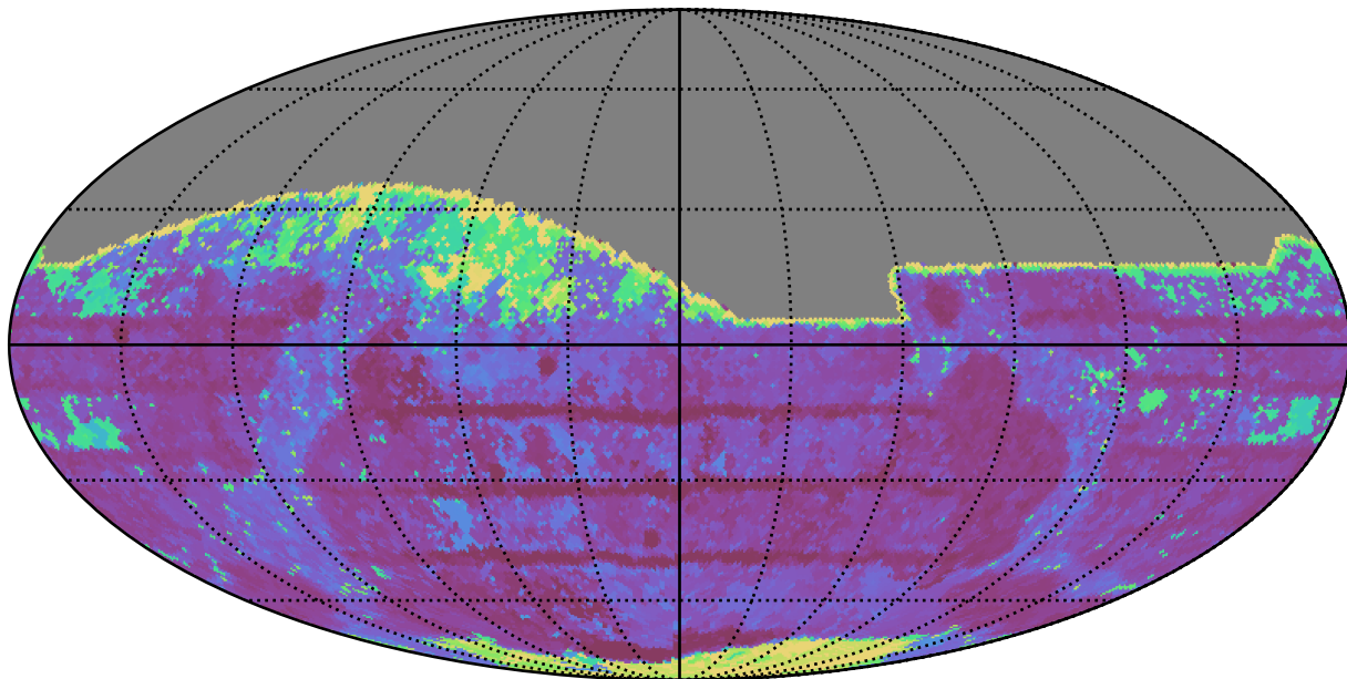
weather_cloudso36v3.4_10yrs All sky z band: Max Inter-Night Gap
