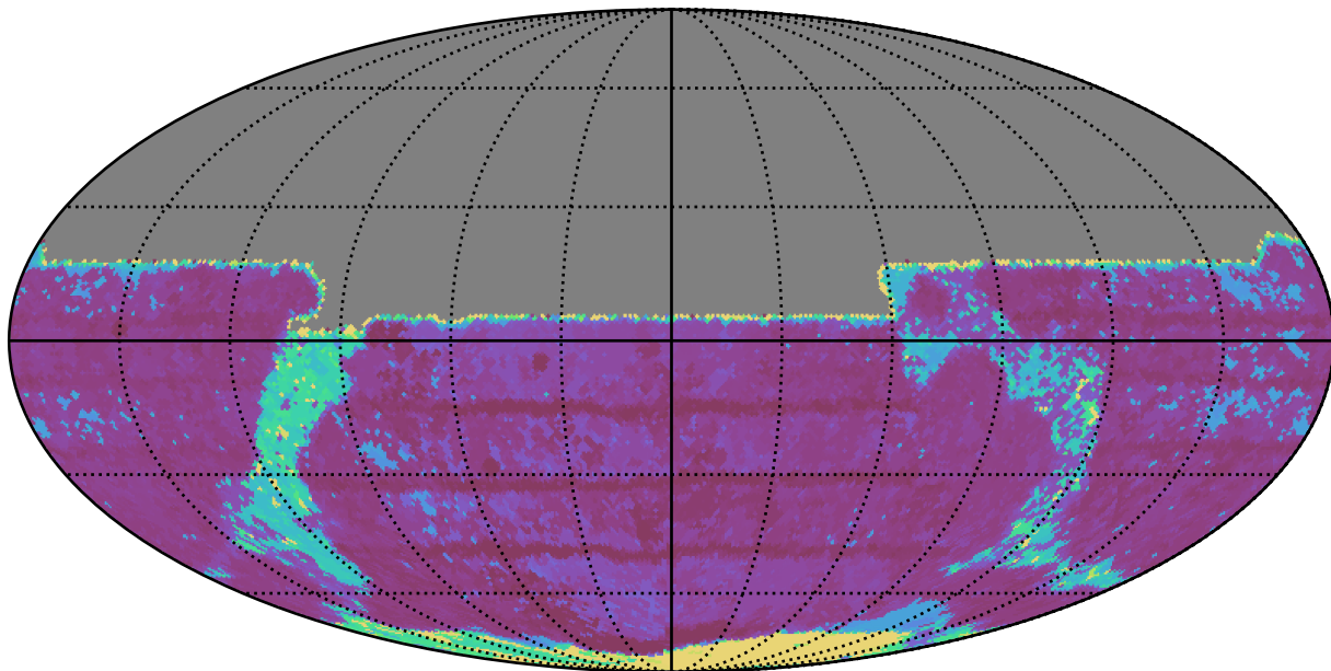
weather_cloudso36v3.4_10yrs All sky y band: Max Inter-Night Gap
