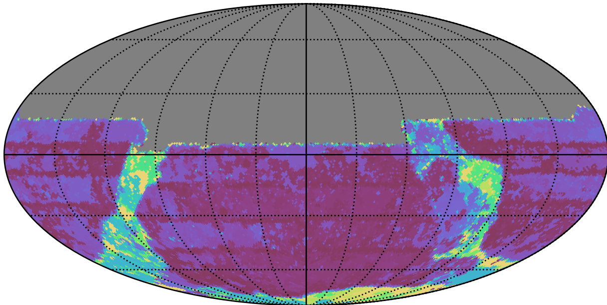
weather_cloudso36v3.4_10yrs All sky u band: Max Inter-Night Gap
