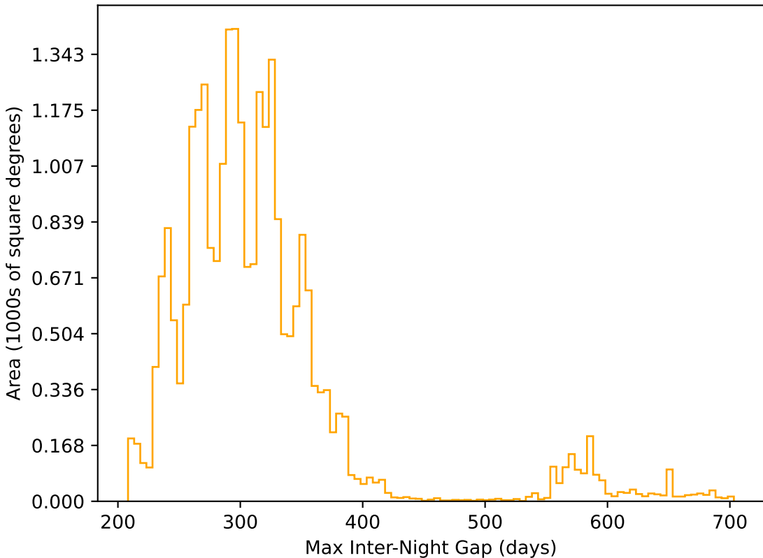
weather_cloudso36v3.4_10yrs All sky r band: Max Inter-Night Gap
