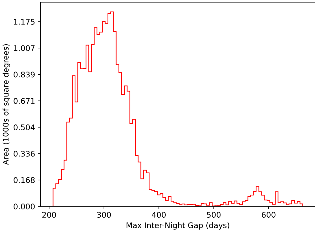
weather_cloudso36v3.4_10yrs All sky i band: Max Inter-Night Gap
