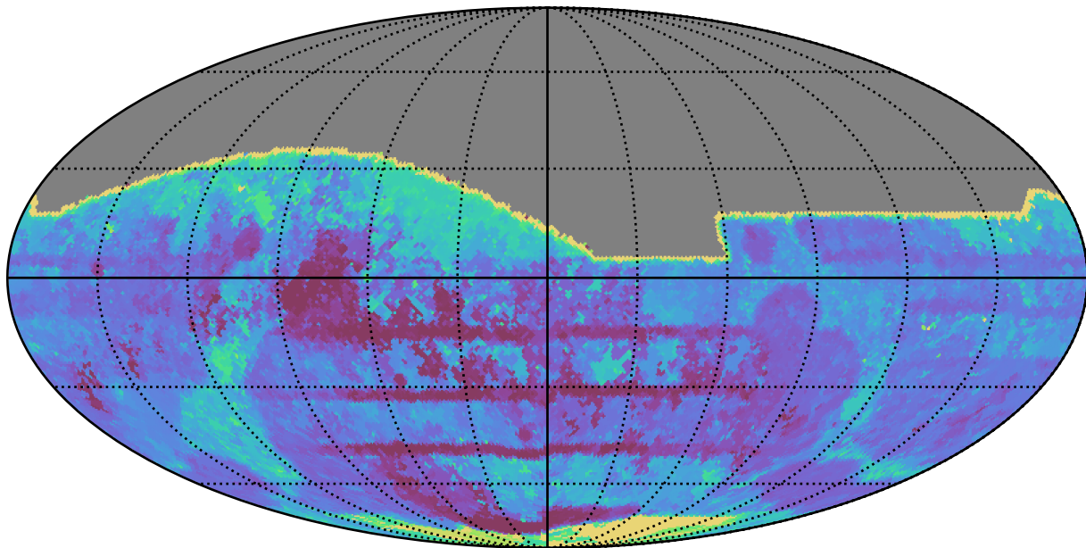
weather_cloudso36v3.4_10yrs All sky all bands: Max Inter-Night Gap
