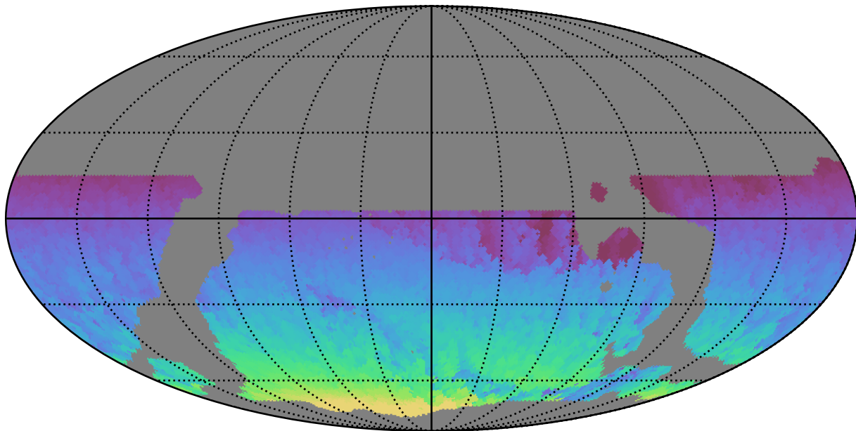
weather_cloudso36v3.4_10yrs WFD all bands: Max HA
