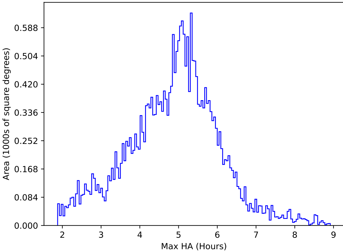
weather_cloudso36v3.4_10yrs All sky all bands: Max HA
