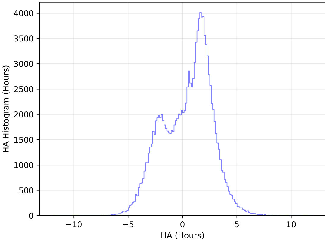
weather_cloudso36v3.4_10yrs WFD u band: HA Histogram
