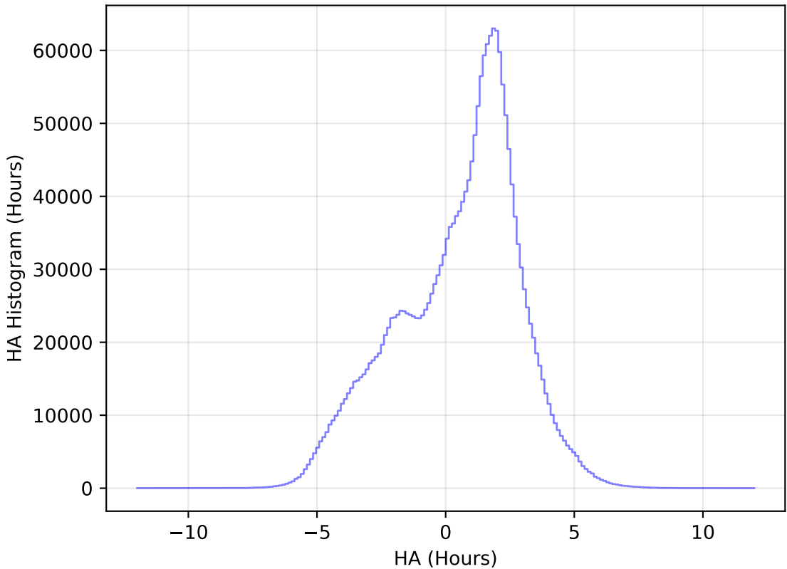
weather_cloudso36v3.4_10yrs WFD all bands: HA Histogram
