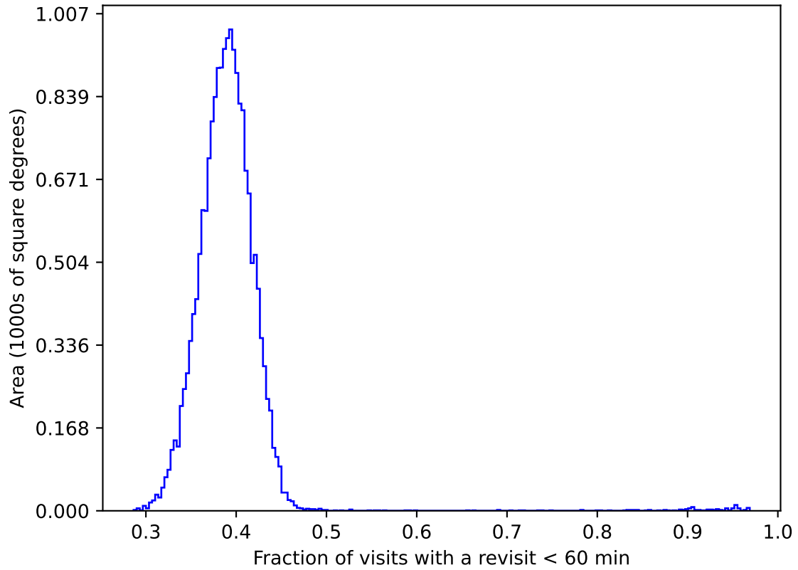
weather_cloudso36v3.4_10yrs gri WFD: Fraction of visits with a revisit < 60 min
