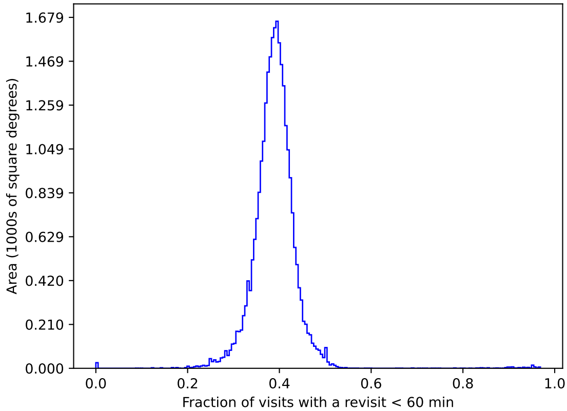
weather_cloudso36v3.4_10yrs gri All sky: Fraction of visits with a revisit < 60 min
