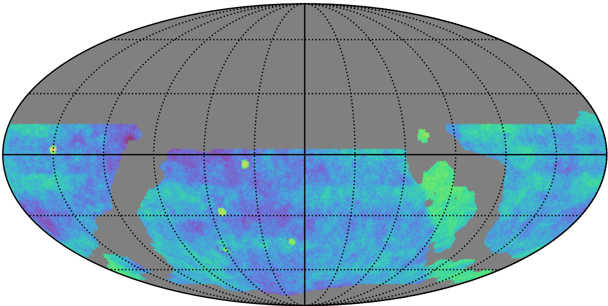
weather_cloudso36v3.4_10yrs gri WFD: Fraction of visits in pairs (20-90 min)
