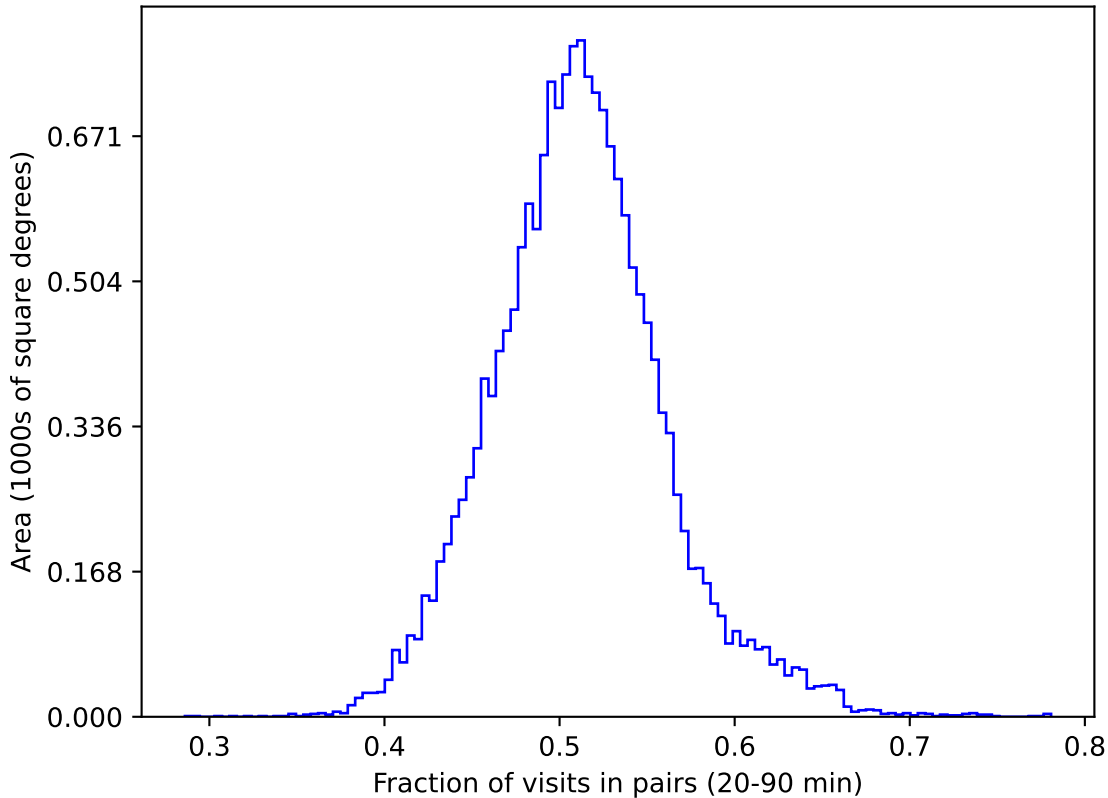
weather_cloudso36v3.4_10yrs gri WFD: Fraction of visits in pairs (20-90 min)
