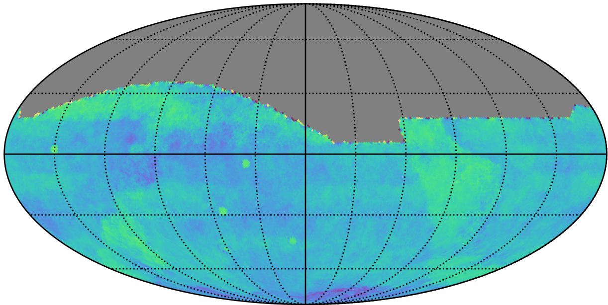
weather_cloudso36v3.4_10yrs gri All sky: Fraction of visits in pairs (20-90 min)
