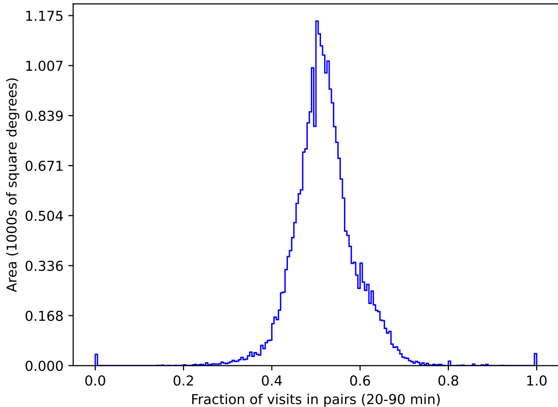
weather_cloudso36v3.4_10yrs gri All sky: Fraction of visits in pairs (20-90 min)
