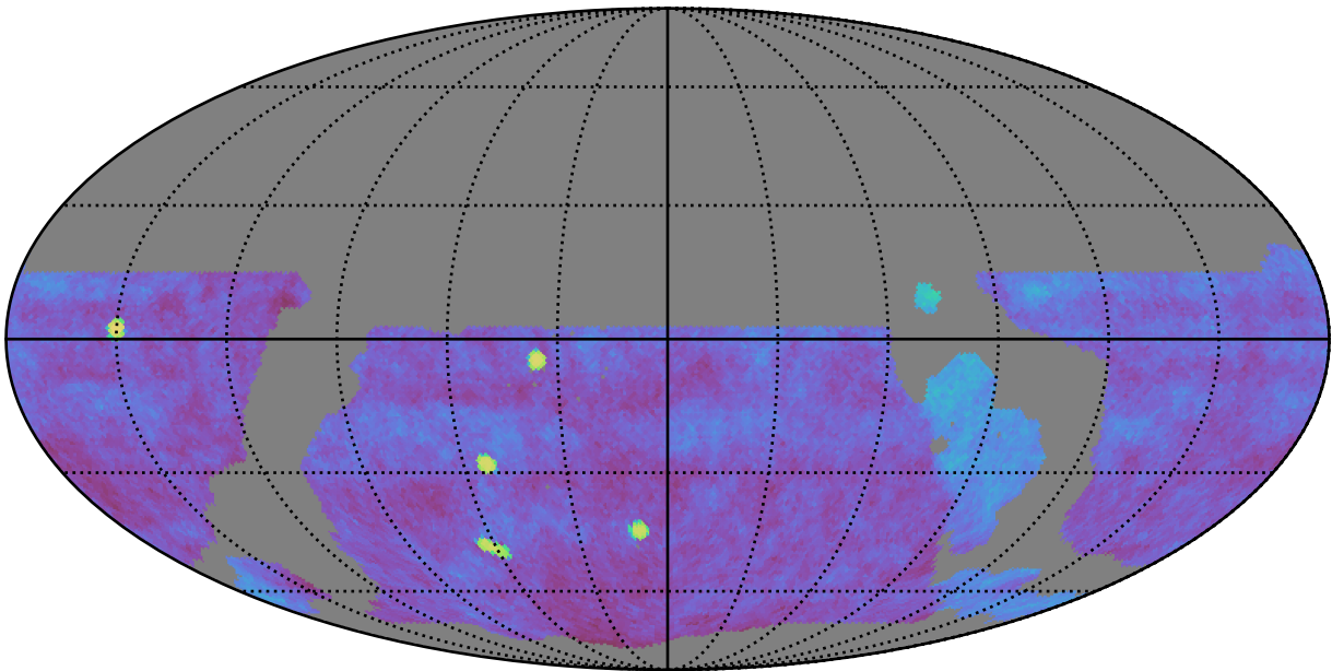
weather_cloudso36v3.4_10yrs gri WFD: Fraction of visits in pairs (10-60 min)
