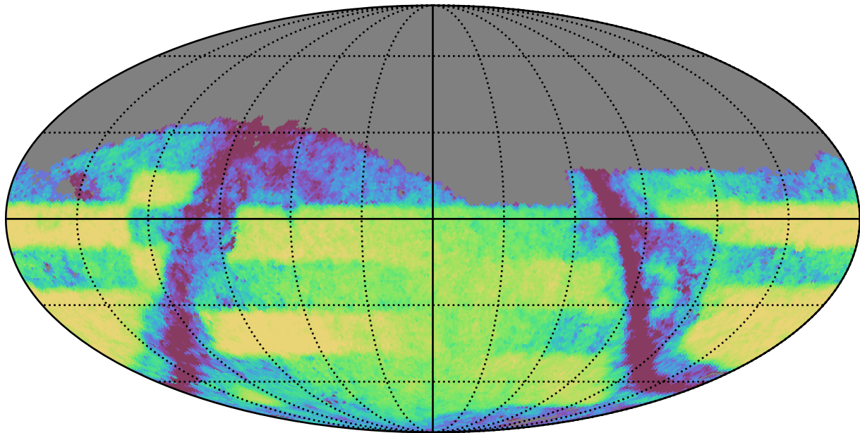
weather_cloudso36v3.4_10yrs Yr 3-4 z band: Exgal_CoaddM5
