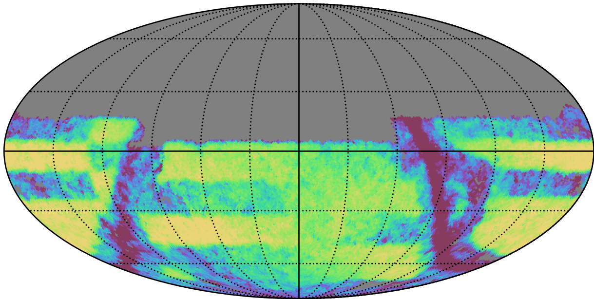
weather_cloudso36v3.4_10yrs Yr 3-4 y band: Exgal_CoaddM5
