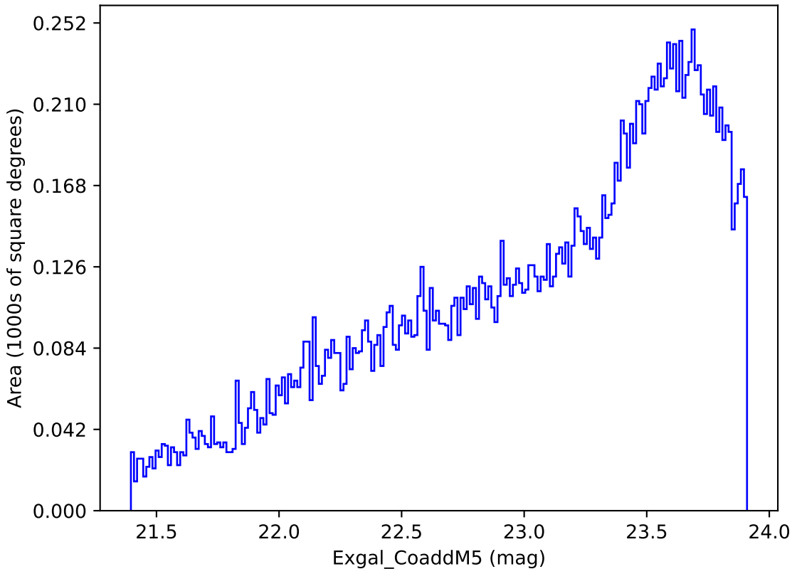
weather_cloudso36v3.4_10yrs Yr 3-4 y band: Exgal_CoaddM5
