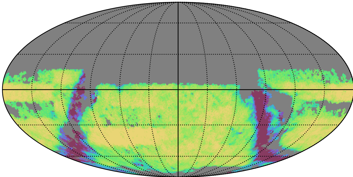
weather_cloudso36v3.4_10yrs Yr 3-4 u band: Exgal_CoaddM5
