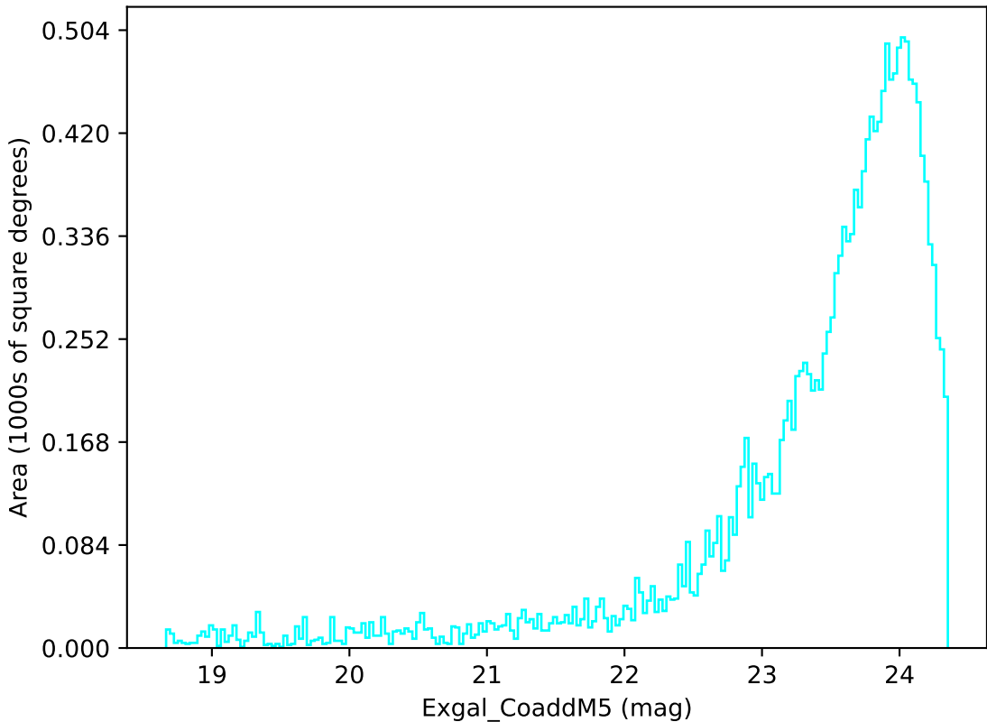
weather_cloudso36v3.4_10yrs Yr 3-4 u band: Exgal_CoaddM5
