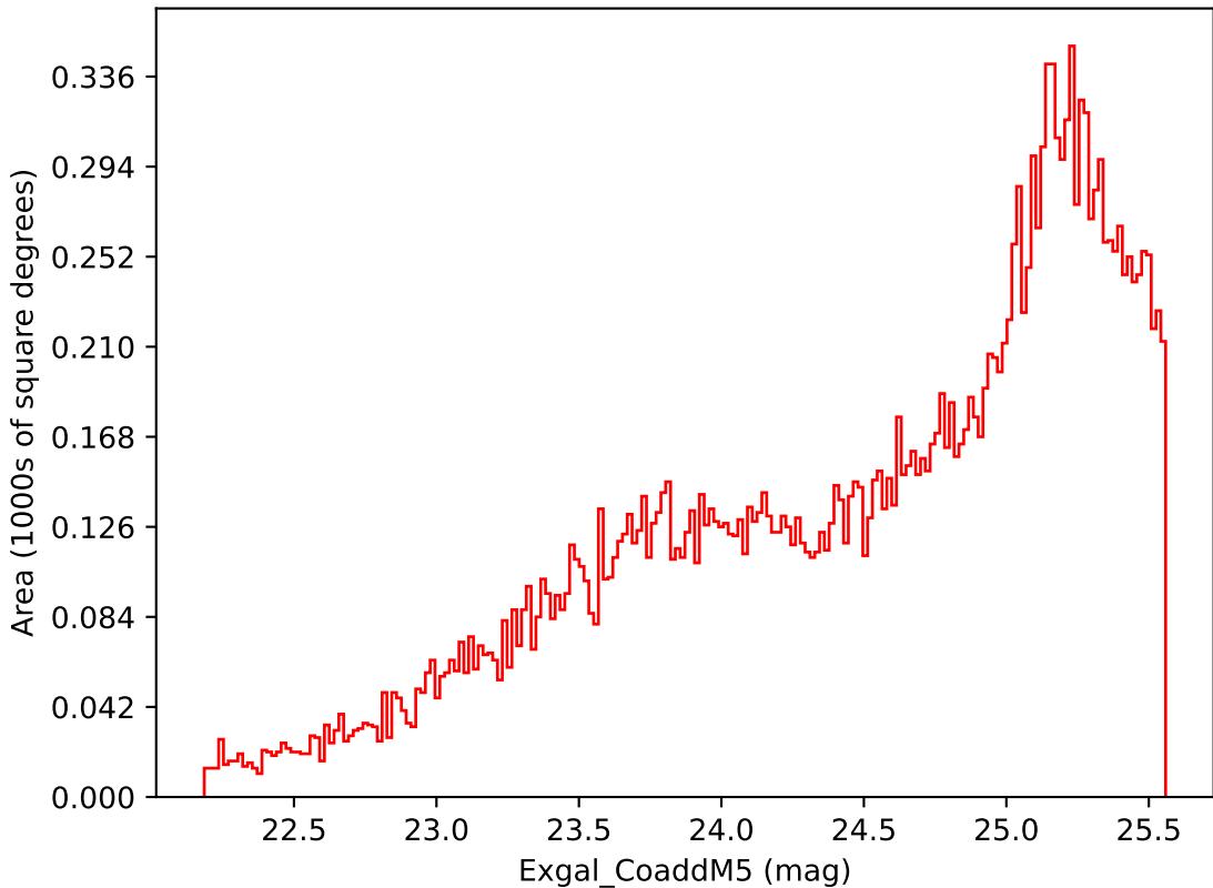
weather_cloudso36v3.4_10yrs Yr 3-4 i band: Exgal_CoaddM5
