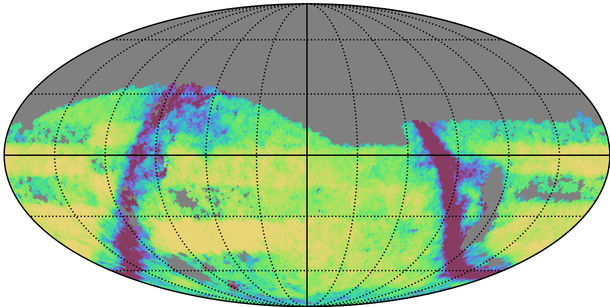
weather_cloudso36v3.4_10yrs Yr 3-4 g band: Exgal_CoaddM5
