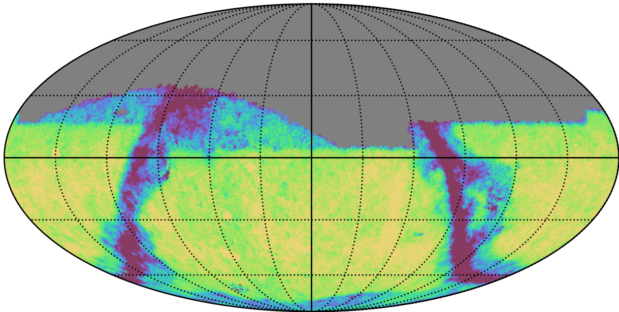
weather_cloudso36v3.4_10yrs Yr 1 z band: Exgal_CoaddM5
