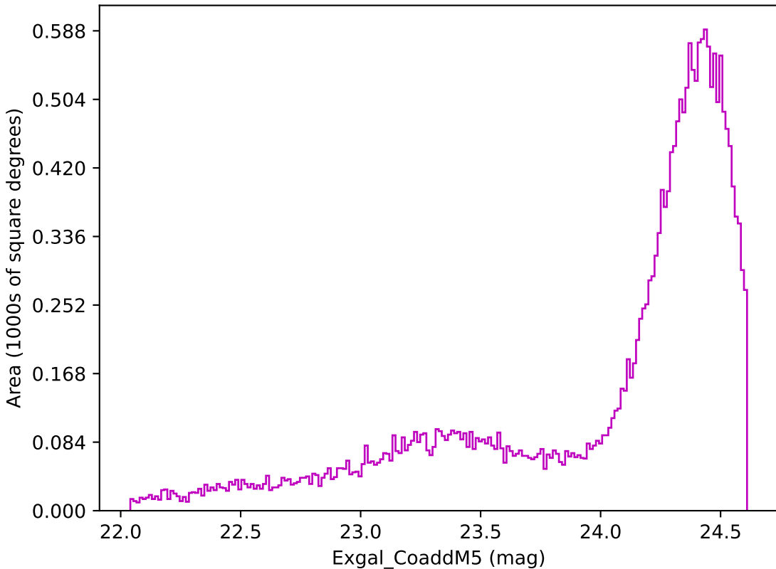
weather_cloudso36v3.4_10yrs Yr 1 z band: Exgal_CoaddM5
