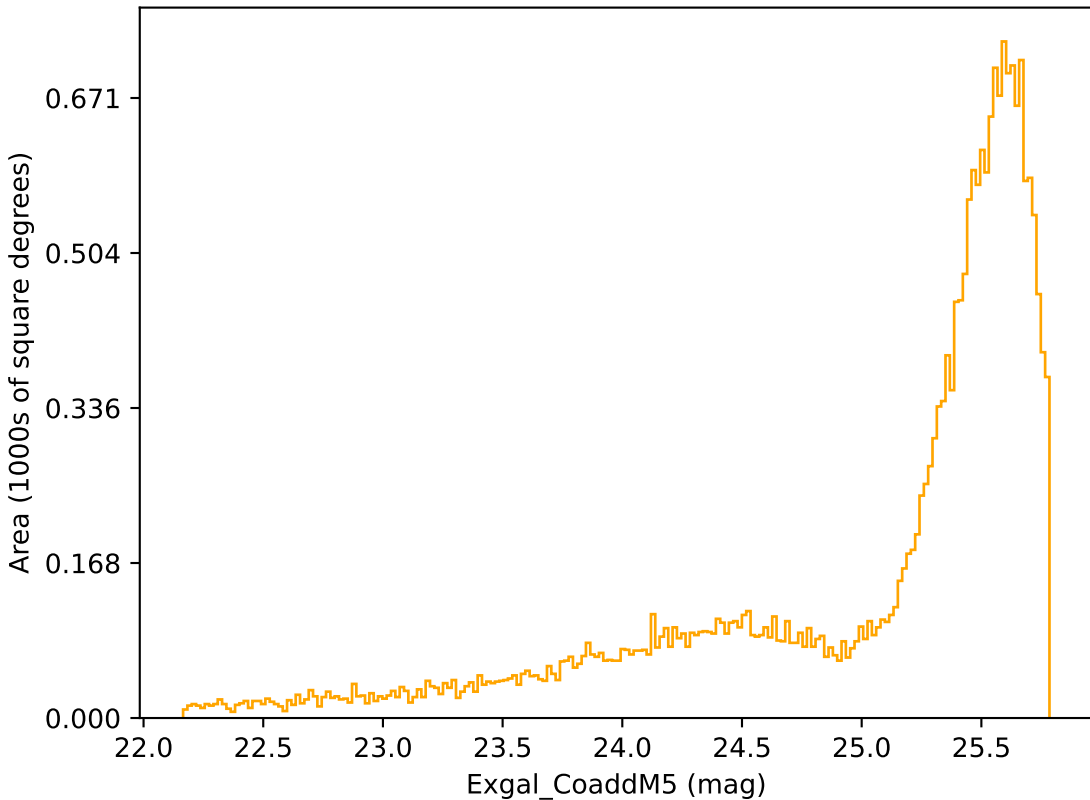
weather_cloudso36v3.4_10yrs Yr 1 r band: Exgal_CoaddM5
